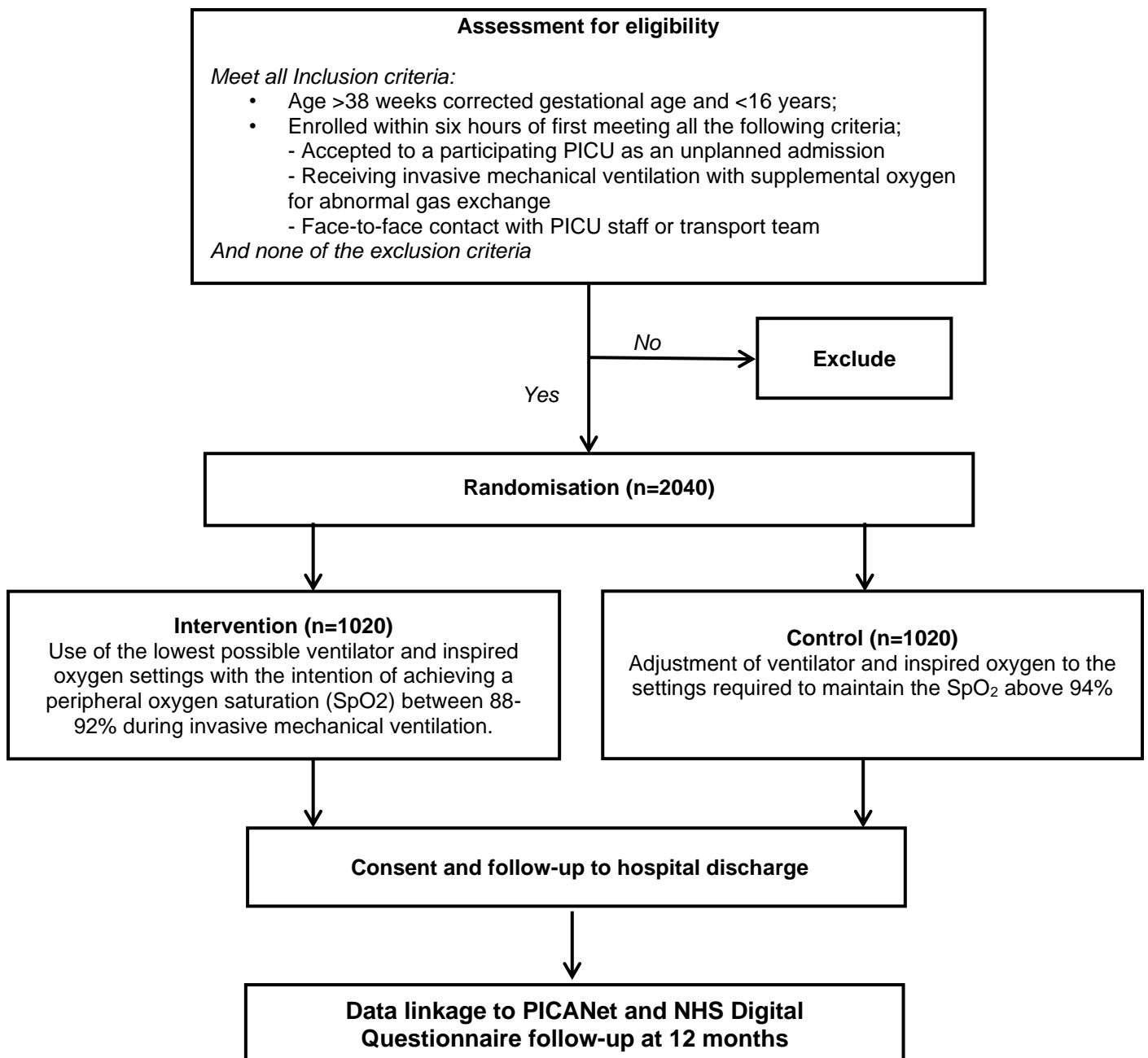
Figure 1 Trial schema
